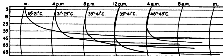
FIG. 21.—Tracing of auxographic records showing swelling of plates of agar 0.18 mm. in thickness at various temperatures. The 5 mm. and 4-hour intervals of the record-slip are shown. Increase is denoted by the downward movement of the pen, which amplifies the actual increase 20 times. The initial and following rates are well illustrated.
